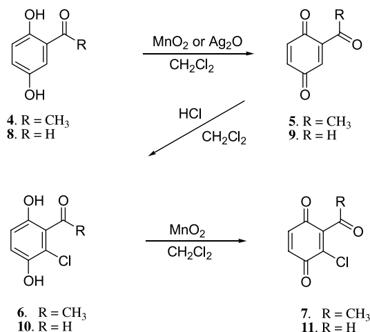
Scheme 1. Synthesis of 2-acyl-3-chloro-1,4-benzoquinones 7 and 11 .
