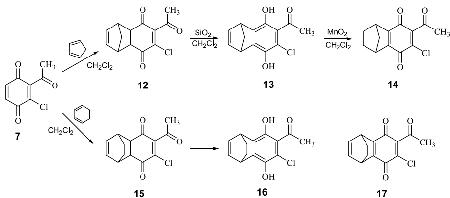
Scheme 2. Synthesis of 6-acetyl-7-chloro-1,4-alkanonaphthalenes 13 , 14 , 16 , and 17 .
